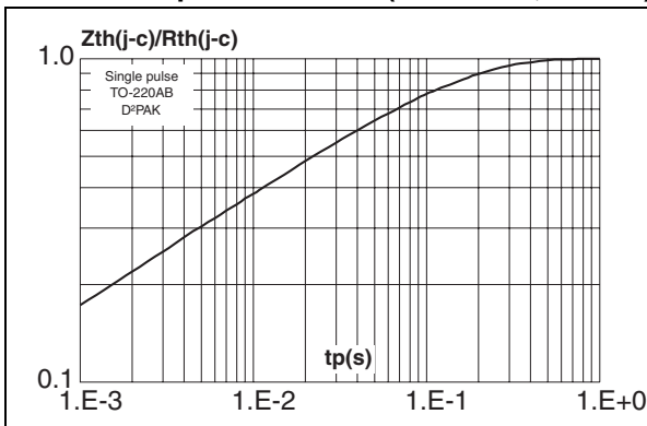
Figure 7. Relative variation of thermal impedance junction to case versus pulse duration (TO-220AB, D²PAK)
